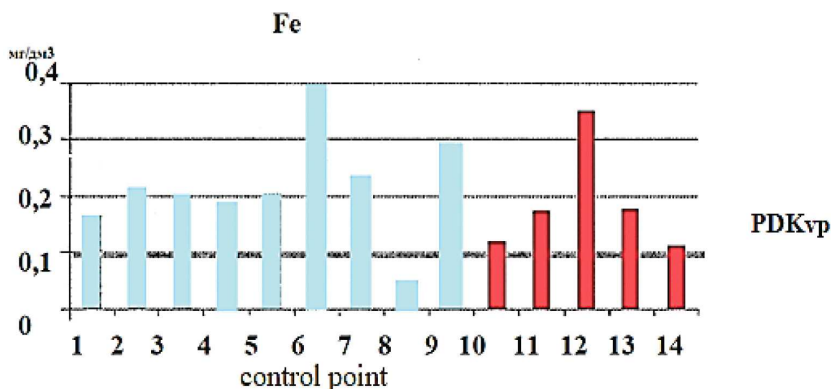
Fig. 3. Exceeding the level of the MPC of iron in the well of the site
