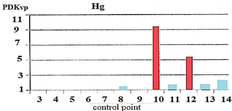
Fig. 6. Excess of the MPC level of mercury in the control points of the site
