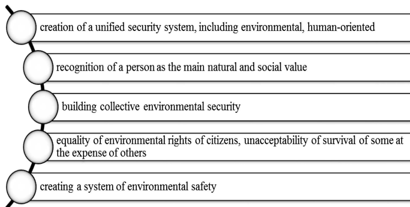
Fig. 2. Elimination of environmental threats
