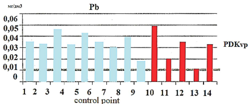
Fig. 4. Excess of the MPC level of lead in the site control point
