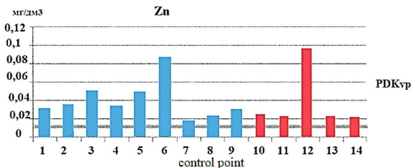
Fig. 7. Excess of the maximum permissible concentration of zinc in the control points of the site
