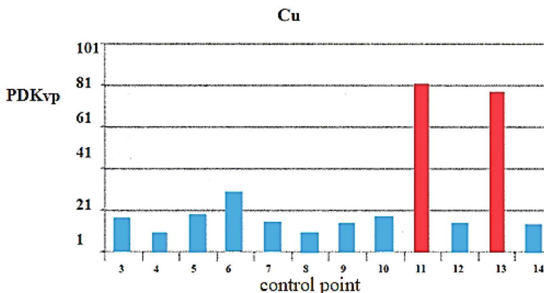
Fig. 5. Excess of the MPC level of copper in the site control point
